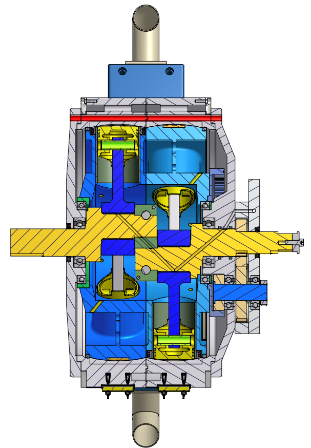
B-B (1:5)
